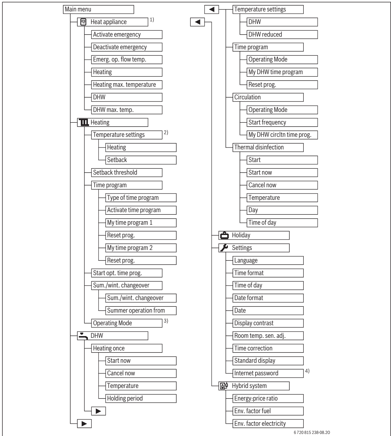
Fig. 3 Menu structure of the main menu
