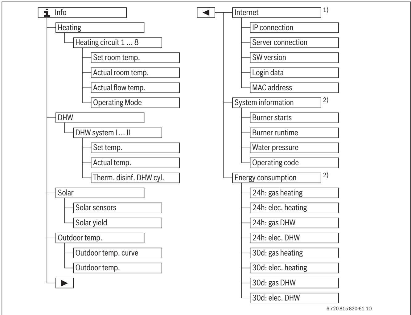
Fig. 5 Menu structure of the info menu
